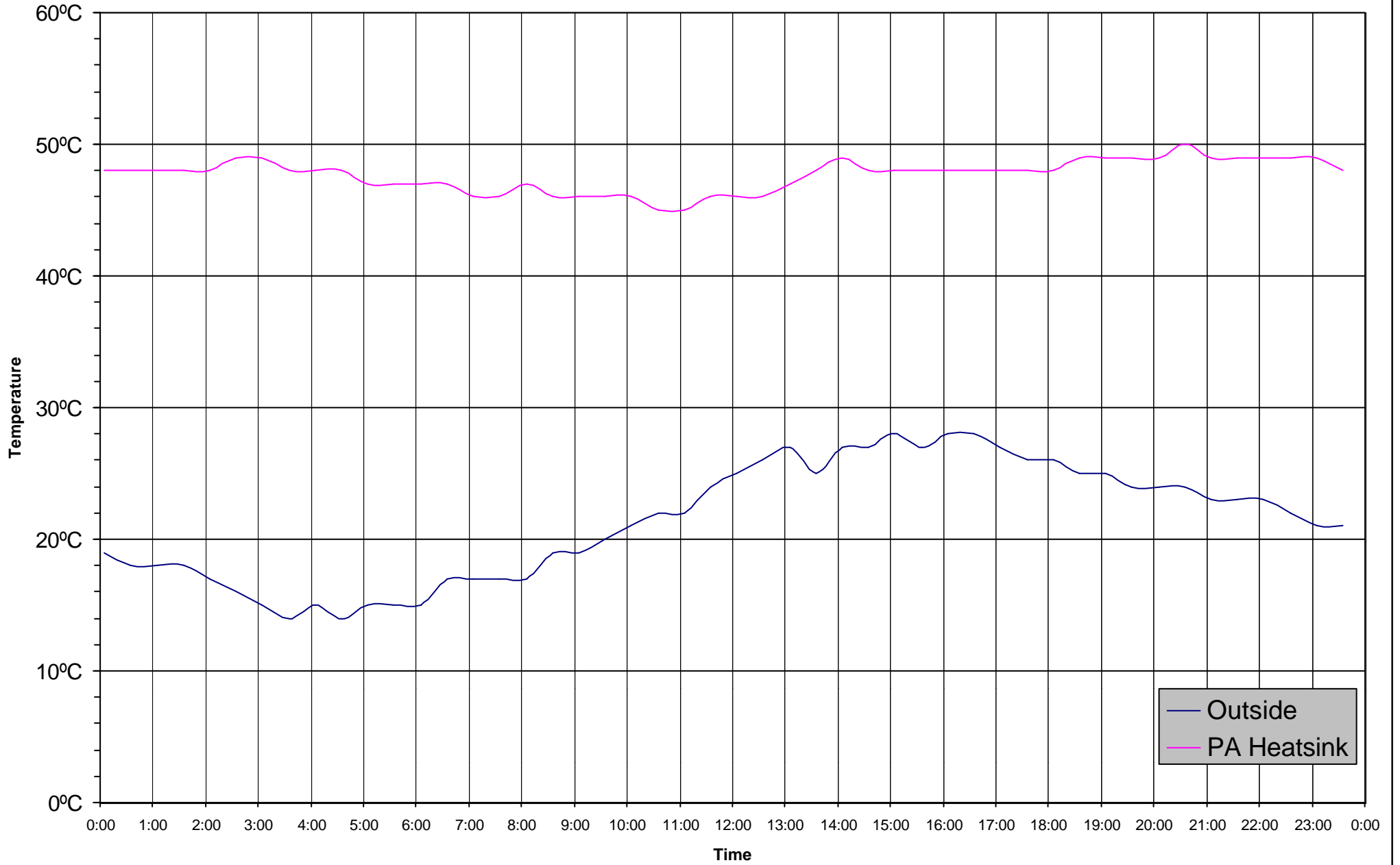
MB7UJ Temperature Sensors - 15th July 2002
